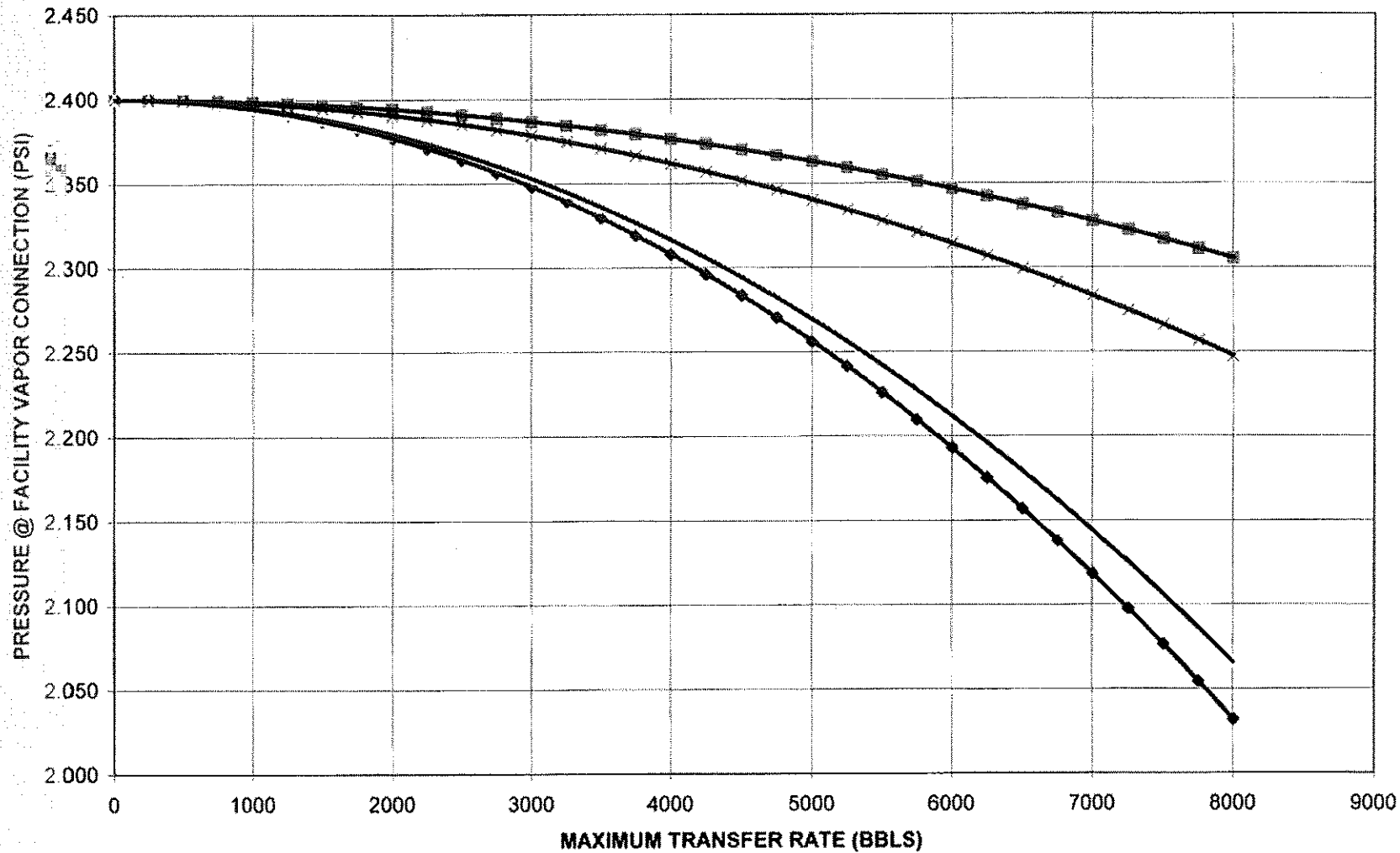
PRESSURE vs MAXIMUM TRANSFER RATE (FOR SUB-CHAPTER "O" CARGOES)
