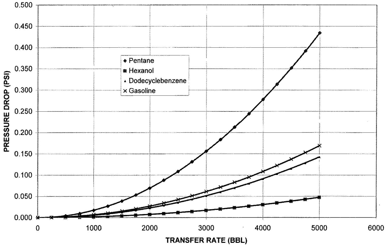
LIQUID TRANSFER RATE vs PRESSURE DROP
