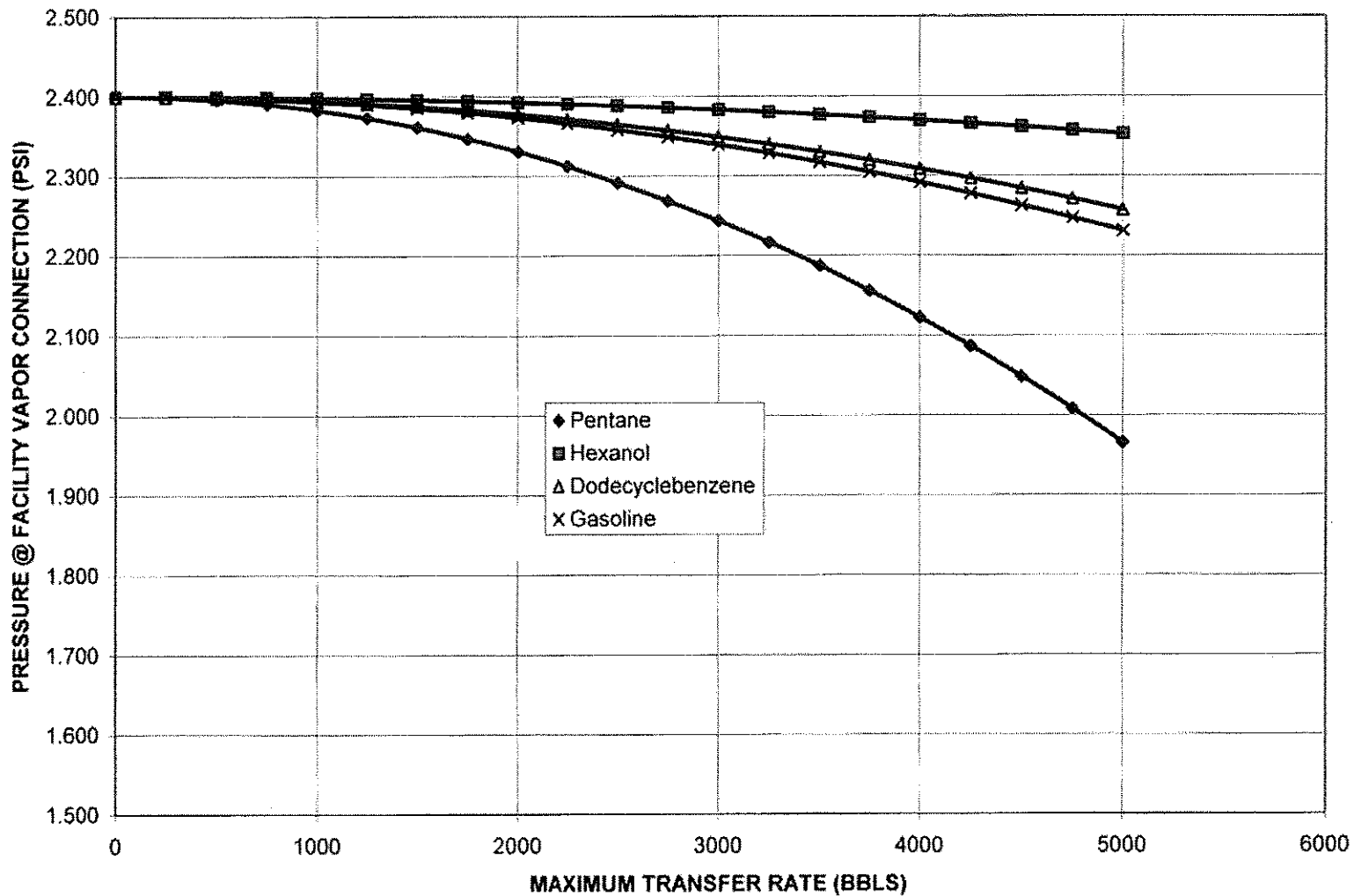
PRESSURE vs MAXIMUM TRANSFER RATE (FOR SUB-CHAPTER "D" CARGOES)
