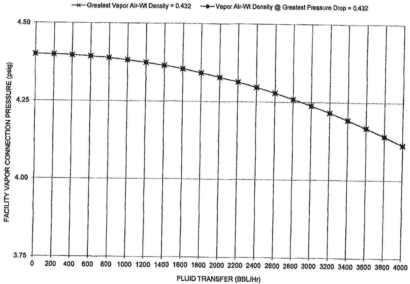
FIG. 2 - Facility Vapor Connection Pressure vs. Maximum Allowable Flowrate based on not Exceeding 80% of the Allowable PV Valve Setting
